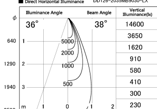
■ Direct Horizontal Illuminance DD126-2035MB9030-LX
