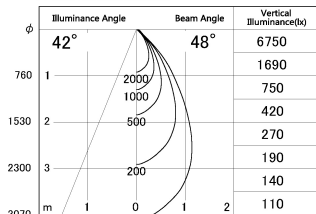
■ Direct Horizontal Illuminance DD126-1455MB9030-LX
