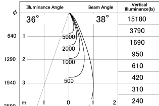
■ Direct Horizontal Illuminance DD126-2035MB9035-LX
