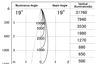
■ Direct Horizontal Illuminance DD126-1415MB9035-LX
