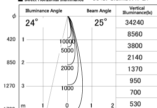
■ Direct Horizontal Illuminance DD126-2025MB9040-LX
