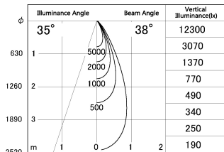
■ Direct Horizontal Illuminance DD126-1435MB9040-LX
