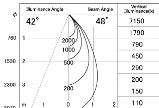
■ Direct Horizontal Illuminance DD126-1455MB9040-LX
