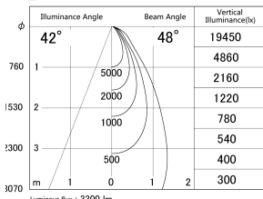
■ Direct Horizontal Illuminance DD146-3050W9027
