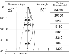
■ Direct Horizontal Illuminance DD146-3525W9027
