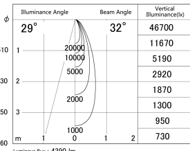
■ Direct Horizontal Illuminance DD146-4035W9027
