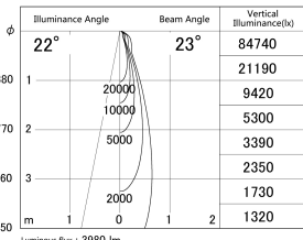
■ Direct Horizontal Illuminance DD146-3525W9030
