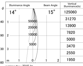
■ Direct Horizontal Illuminance DD146-4015W9030
