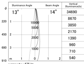
Direct Horizontal Illuminance DD146-0815W9035
