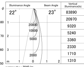
■ Direct Horizontal Illuminance DD146-3525W9035
