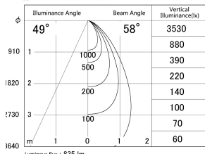
■ Direct Horizontal Illuminance DD146-0850W9040
