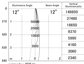
■ Direct Horizontal Illuminance DD146-2015W9040
