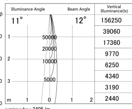
■ Direct Horizontal Illuminance DD146-2515W9040
