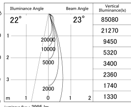
■ Direct Horizontal Illuminance DD146-3525W9040
