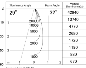
■ Direct Horizontal Illuminance DD146-3535W9040
