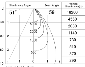
■ Direct Horizontal Illuminance DD146-4050W9040
