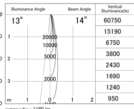
■ Direct Horizontal Illuminance DD146-1515B9027
