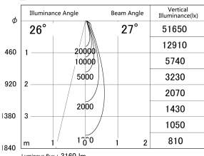
■ Direct Horizontal Illuminance DD146-2525B9030
