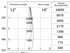
Direct Horizontal Illuminance DD146-0815B9035
