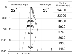
■ Direct Horizontal Illuminance DD146-4025B9040
