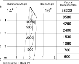
■ Direct Horizontal Illuminance DD139-1515MW9027
