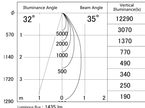
■ Direct Horizontal Illuminance DD139-1530MW9027
