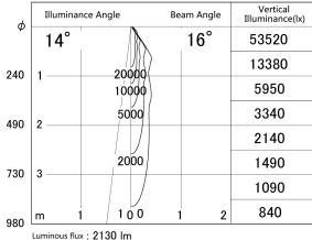
■ Direct Horizontal Illuminance DD139-2015MW9027
