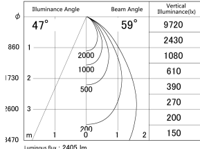
■ Direct Horizontal Illuminance DD139-2550MW9027
