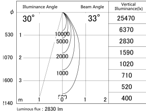
■ Direct Horizontal Illuminance DD139-3030MW9027
