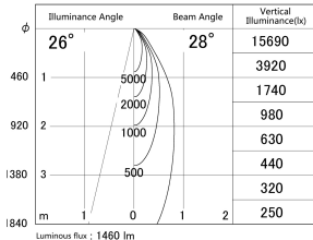
■ Direct Horizontal Illuminance DD139-1520MW9030
