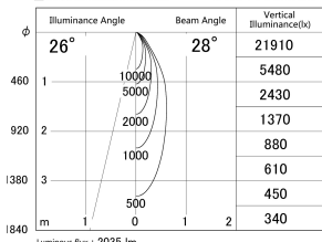
■ Direct Horizontal Illuminance DD139-2020MW9030
