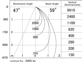
■ Direct Horizontal Illuminance DD139-2550MW9030
