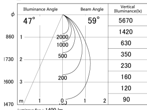
■ Direct Horizontal Illuminance DD139-1550MW9035
