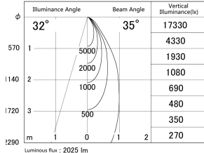
■ Direct Horizontal Illuminance DD139-2030MW9035
