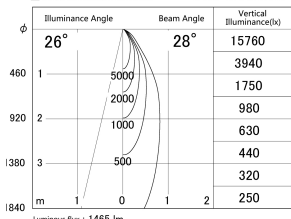
■ Direct Horizontal Illuminance DD139-1520MW9040
