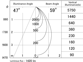
■ Direct Horizontal Illuminance DD139-1550MW9040
