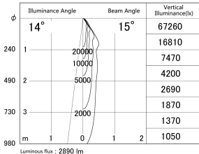
■ Direct Horizontal Illuminance DD139-3015MW9040
