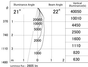
■ Direct Horizontal Illuminance DD139-2520MB9027
