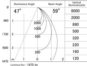
■ Direct Horizontal Illuminance DD139-2050MB9030
