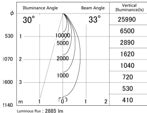
■ Direct Horizontal Illuminance DD139-3030MB9030
