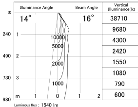
■ Direct Horizontal Illuminance DD139-1515MB9035
