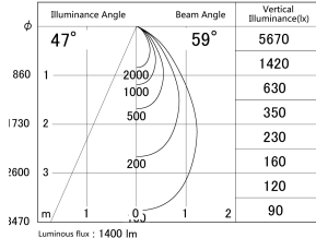
■ Direct Horizontal Illuminance DD139-1550MB9035
