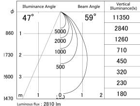
■ Direct Horizontal Illuminance DD139-3050MB9035
