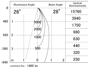
■ Direct Horizontal Illuminance DD139-1520MB9040
