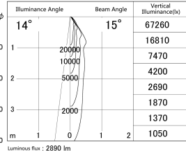
■ Direct Horizontal Illuminance DD139-3015MB9040
