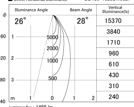
■ Direct Horizontal Illuminance DD139-1520DW9027
