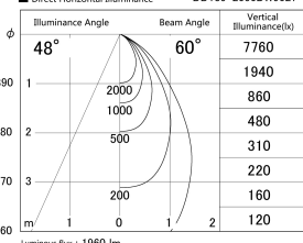
■ Direct Horizontal Illuminance DD139-2050DW9027
