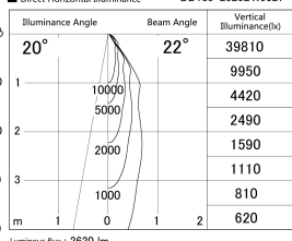
■ Direct Horizontal Illuminance DD139-2520DW9027
