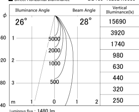
■ Direct Horizontal Illuminance DD139-1520DW9030
