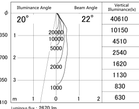
■ Direct Horizontal Illuminance DD139-2520DW9030
